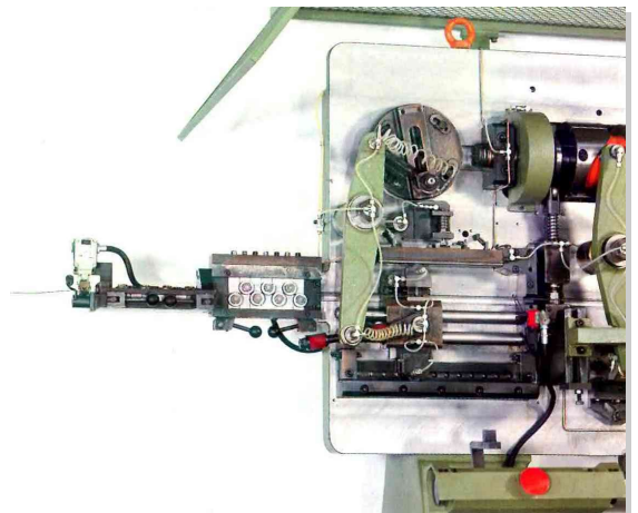
Straightener and mechanical feed device with grippers
